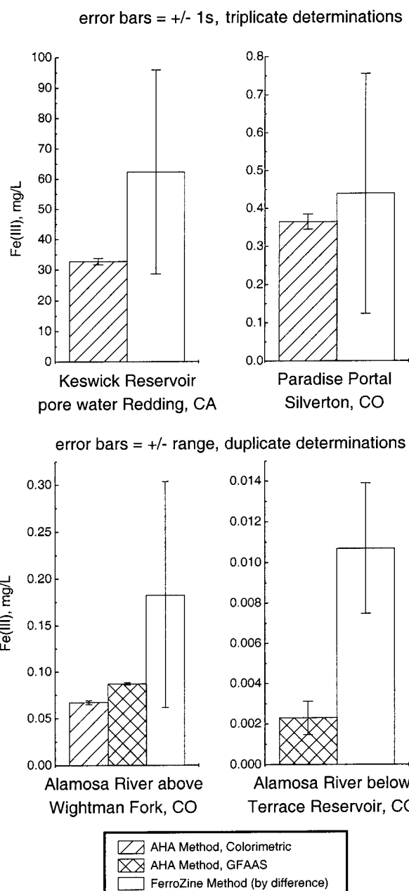
FIGURE 7. Comparison of Fe(III) concentrations determined directly using the acetohydroxamic acid (AHA) method with Fe(III) concentrations determined by difference using the FerroZine method.
